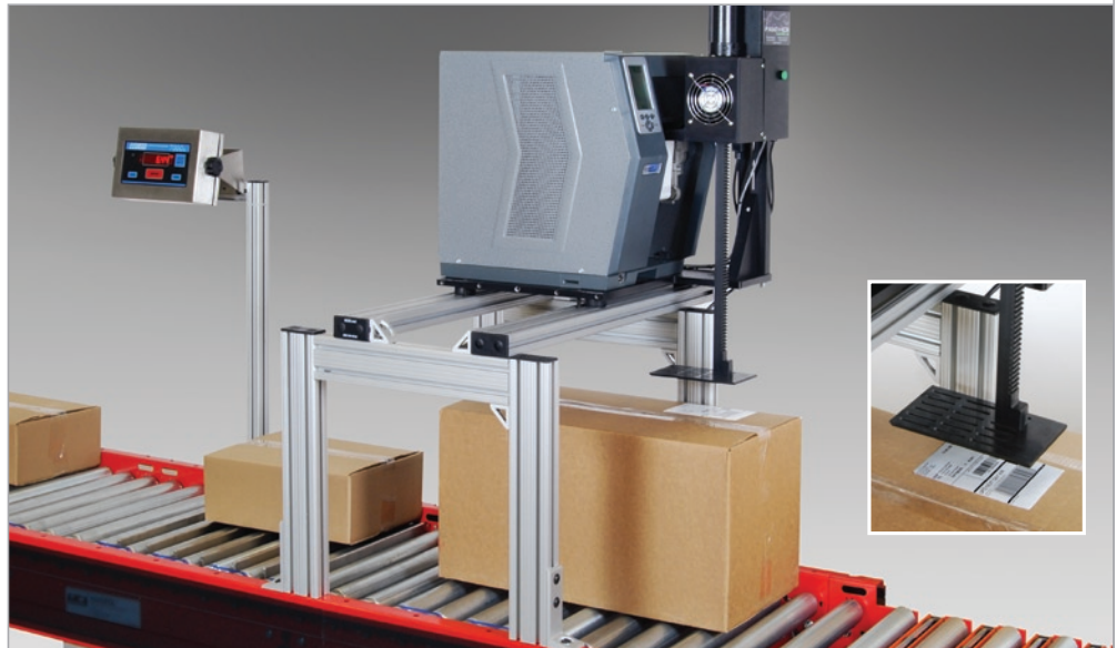
Automate Packing, Shipping, and Manifesting at rates of 750-plus cartons per hour for FedEx, UPS and USPS.
